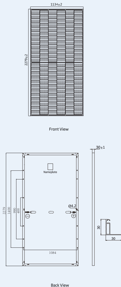
Dimensions of PV Module (Unit: mm)
