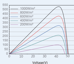
P-V Curves of PV Module (535W)
